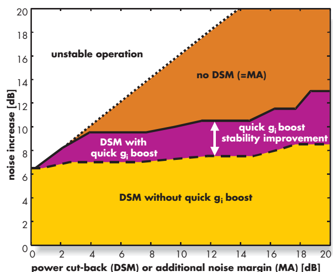
Figure 8: Improving stability by introducing the quick g_i boost when applying DSM. Note that the horizontal scale has a different meaning for DSM and for MA mode: PCB for DSM (dashed line and full line) and additional noise margin for MA mode (dotted line).
