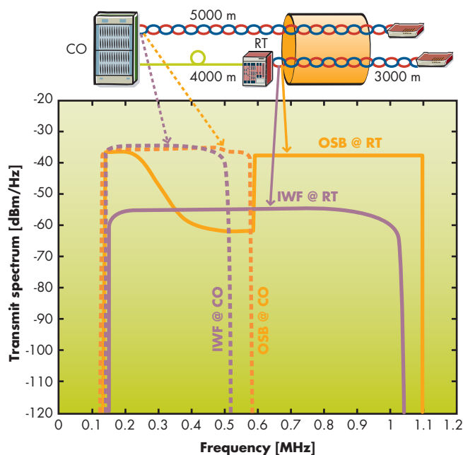
Figure 2: IWF and OSB transmit spectra for a case of mixed CO/RT deployment.
