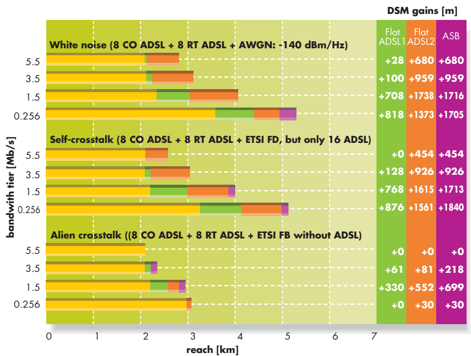
Figure 5: DSM level 1 performance on the CO lines for mixed CO/RT-fed ADSL MA (yellow), ADSL1 flat power back-off (green), ADSL2 flat power back-off (orange), Autonomous Spectrum Balancing (purple).
