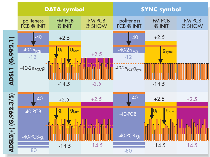
Figure 9: Transmit power control in ADSL1 and ADSL2(+)
