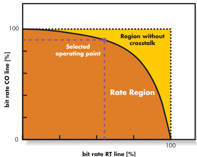
Figure 6: Rate region and trade-off between CO-RT bit rate
