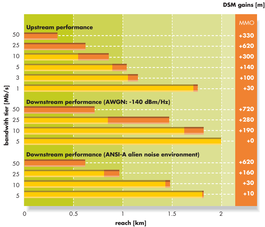
Figure 7: DSM level 3 performance gains for VDSL
