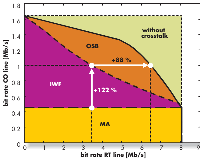
Figure 3: Rate region of a CO and RT line operating in MA mode (yellow), applying IWF (purple), and OSB (orange).
